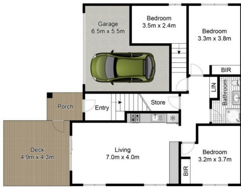
Lower Duplex
